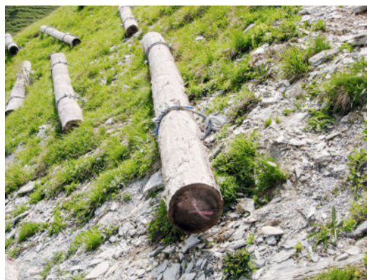
Figure 57 Wooden logs anchored with two wire rope anchors. The advantage of wire rope anchoring is that the logs can be replaced more easily if required.
