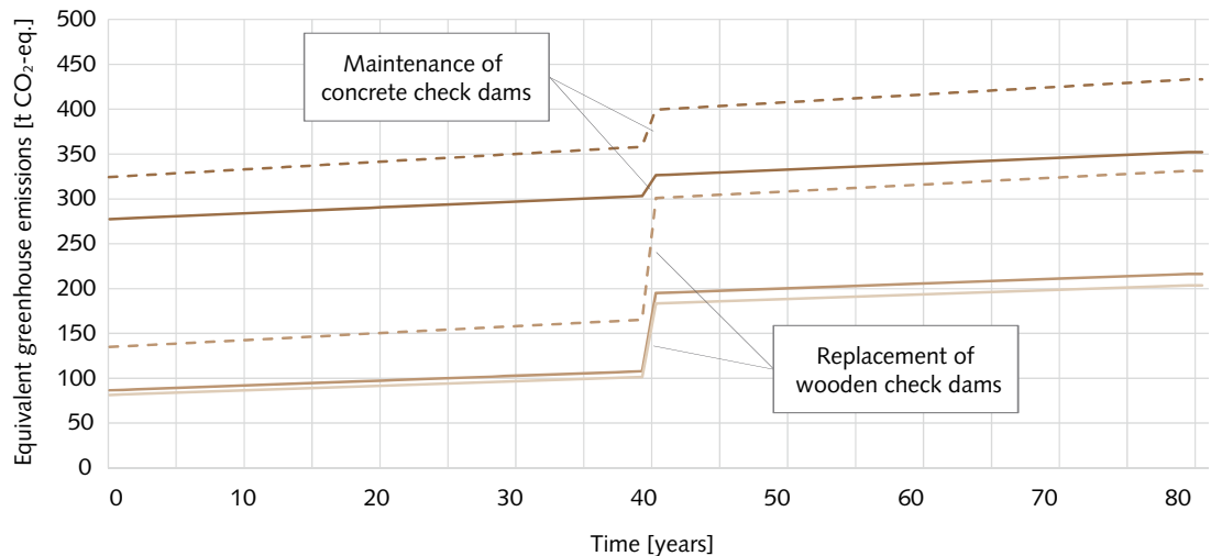
Figure 66 Greenhouse gas emissions over 80 years for concrete and wooden variants B1 and H1 (actual transport distances) and of variants B2 and H2 (extended transport distances) and variant H3 (shorter transport distances due to use of regionally sourced timber) [65].
