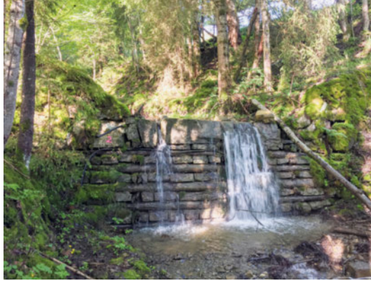
Figure 67 Check dam in the Schaferabach stream in the municipality of Plaffeien, Switzerland. Some of the dams in the Schaferabach are known to have been built between 1940 and 1945. This means they have served unaltered for more than 75 years.
