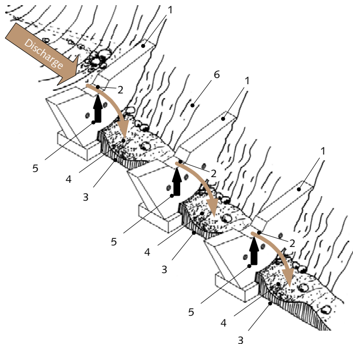
Figure 33 Schematic diagram of the stabilisation function achieved by means of a chain of check dams.
