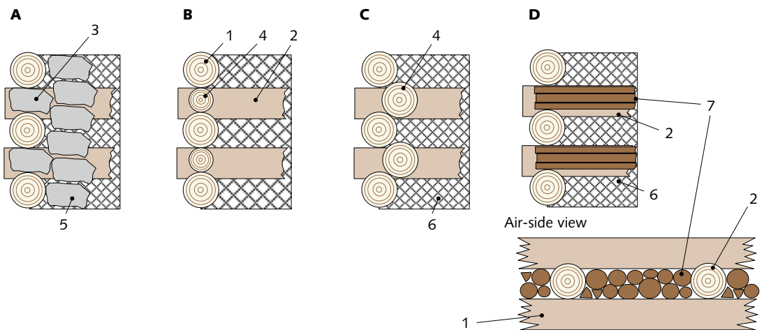
Figure 36 Infill of cribwalls. Detail from Figure 35.
